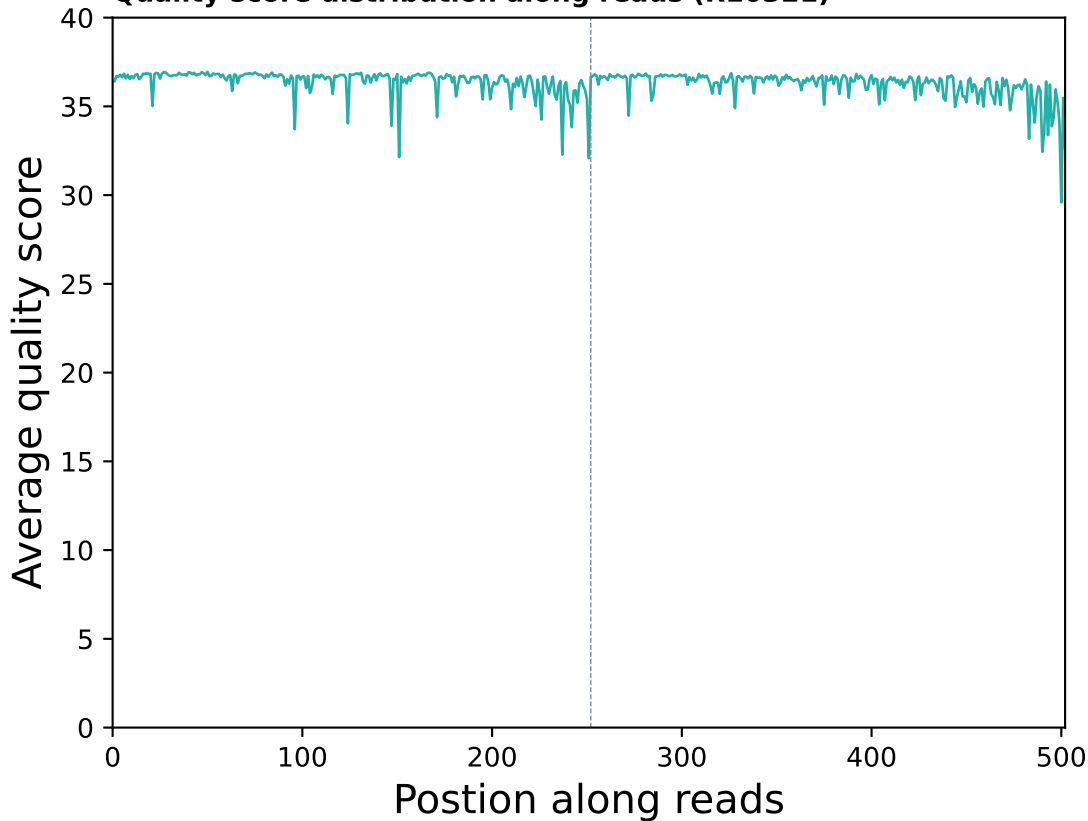
Quality score distribution along reads (R10321)
